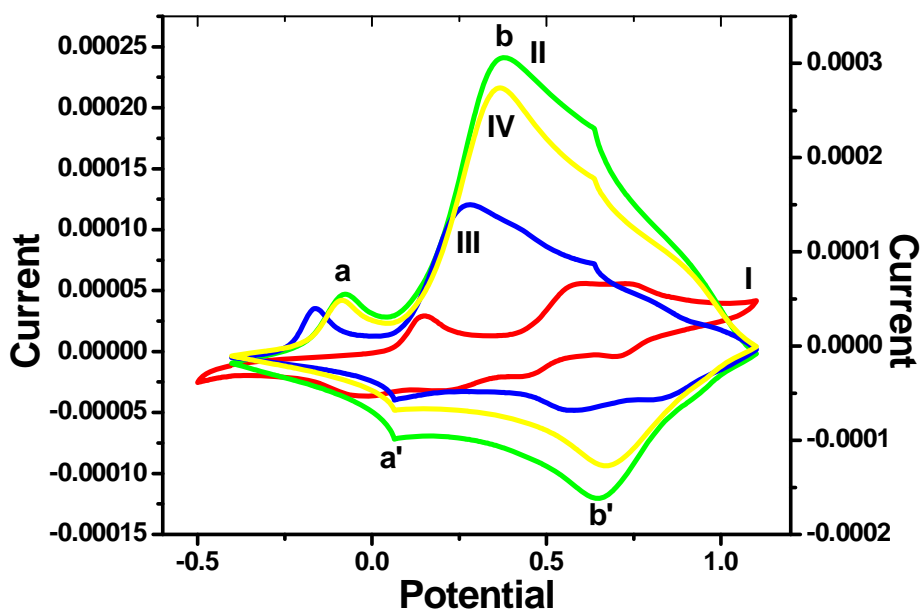
Fig. 3. Cyclic Voltammogram of nanostructured conducting polyaniline (I) S4; (II) D2;(III) SC3; (IV) DC2
