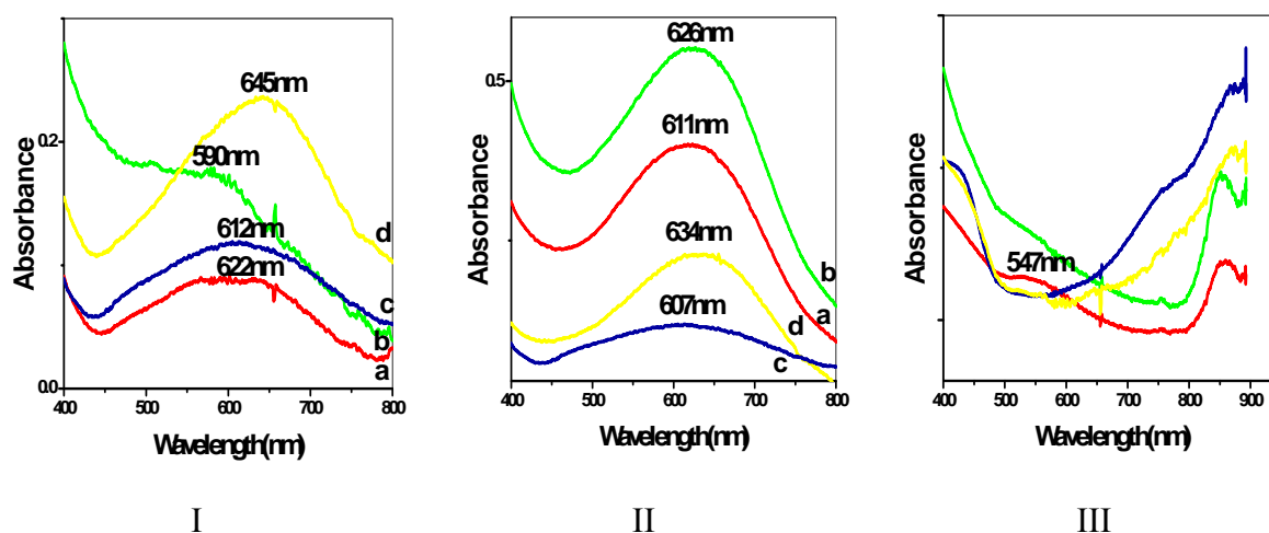
Fig. 5. UV-Vis spectra of nanostructured conducting polyaniline after treating with (I) NMP;(II)DMSO;(III) DMF (a=S4,b=D2,c=SC3,d=DC2)
