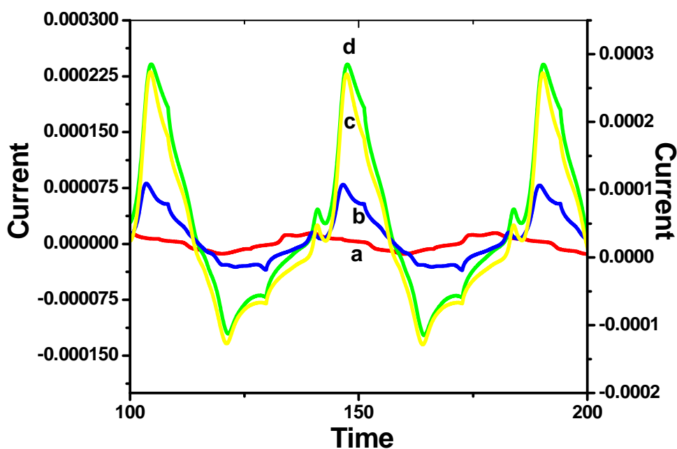
Fig. 4. Current vs. Time plot of nanostructured conducting polyaniline(a) S4;(b) D2;(c) SC3;(d) DC2
