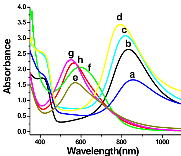
Fig. 1. UV-Vis spectra of nanostructured conducting polyaniline (a) D2(doped);(b) S4(doped); (c) SC3(doped); (d) DC2(doped); (e) S4(undoped); (f) D2(undoped); (g) SC3 (dedoped); (h) DC2(dedoped)
