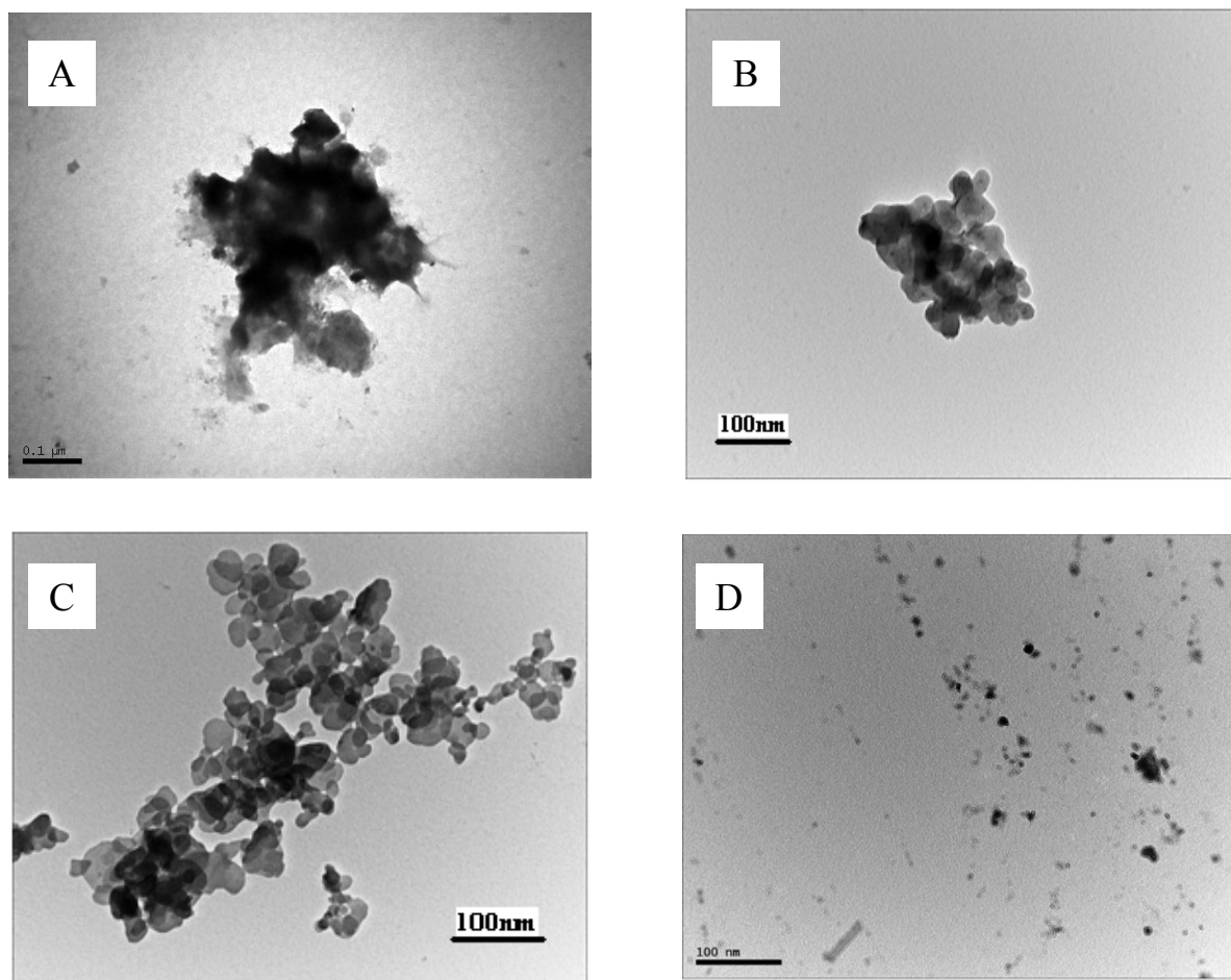
Fig. 2. TEM images of (a) S4(Undoped) (b) S4(Dedoped) (c) D2(Undoped) (d) D2(Dedoped)
