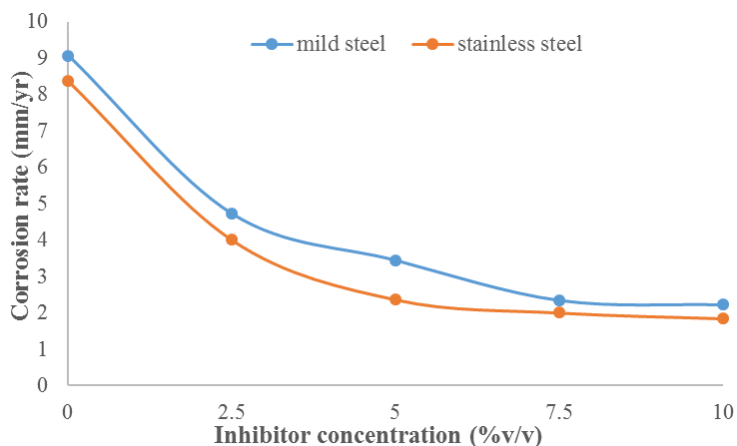
Fig. 6. Corrosion rate of A315 mild steel and 304 stainless steel samples in acidic medium with varied concentrations of natural honey inhibitor
