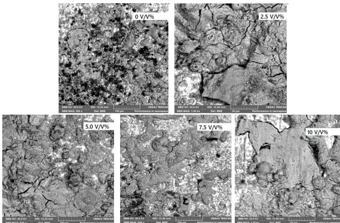
Fig. 8. SEM analysis of the surfaces of the mild steel
