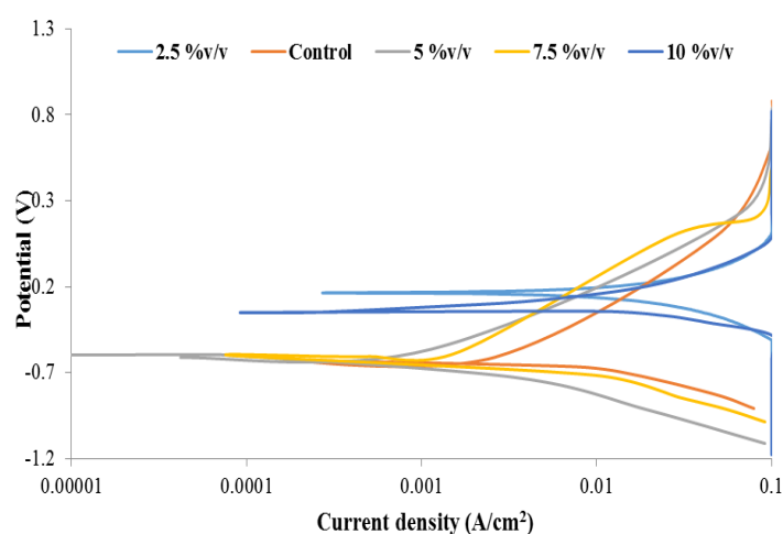
Fig. 4. Tafel plots for A315 mild steel in acidic medium with varied concentrations of natural honey inhibitor
