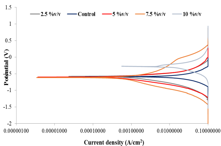
Fig. 5. Tafel plots for 304 stainless steel in acidic medium with varied concentrations of natural honey inhibitor
