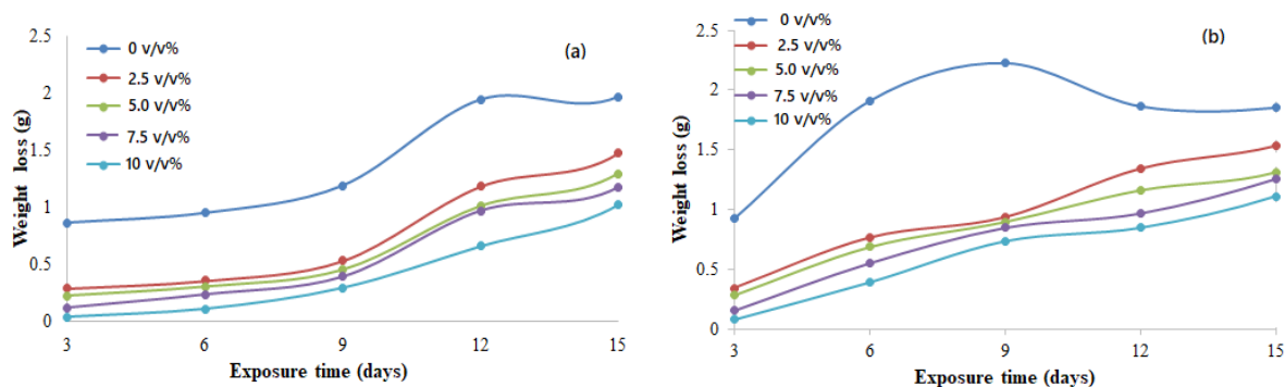
Fig. 2. Trends of the weight loss observed for (a) mild steel and (b) stainless steel samples
