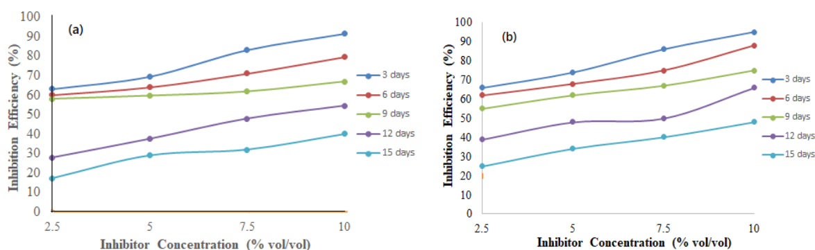
Fig. 3 Inhibition efficiency of (a) mild steel and (b) stainless steel
