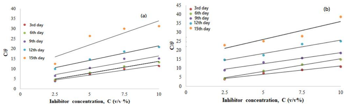
Fig. 7. Plots of C/\theta versus C for mild steel and stainless steel
