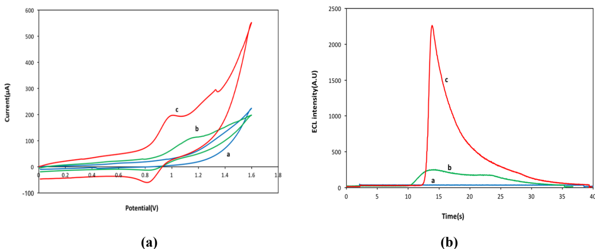
Fig. 4. (a) Cyclic voltammograms GCE(a), \text{Ru}(\text{bpy})_3^{2+} -GCE(b), \text{Sm}_2\text{O}_3 NPs- \text{Ru}(\text{bpy})_3^{2+} -GCE(c). supporting electrolyte buffer solution (0.1 M and pH 8.5) and 5 \times 10^{-8} M Phenylalanine; potential scan rate, 100 \text{ mV s}^{-1} ; (b) ECL responses of GCE(a), \text{Ru}(\text{bpy})_3^{2+} -GCE(b), \text{Sm}_2\text{O}_3 NPs- \text{Ru}(\text{bpy})_3^{2+} -GCE(c) in 0.1 M pH 8.5 phosphate buffer containing 5 \times 10^{-8} M Phenylalanine; potential scan rate, 100 \text{ mV s}^{-1}
